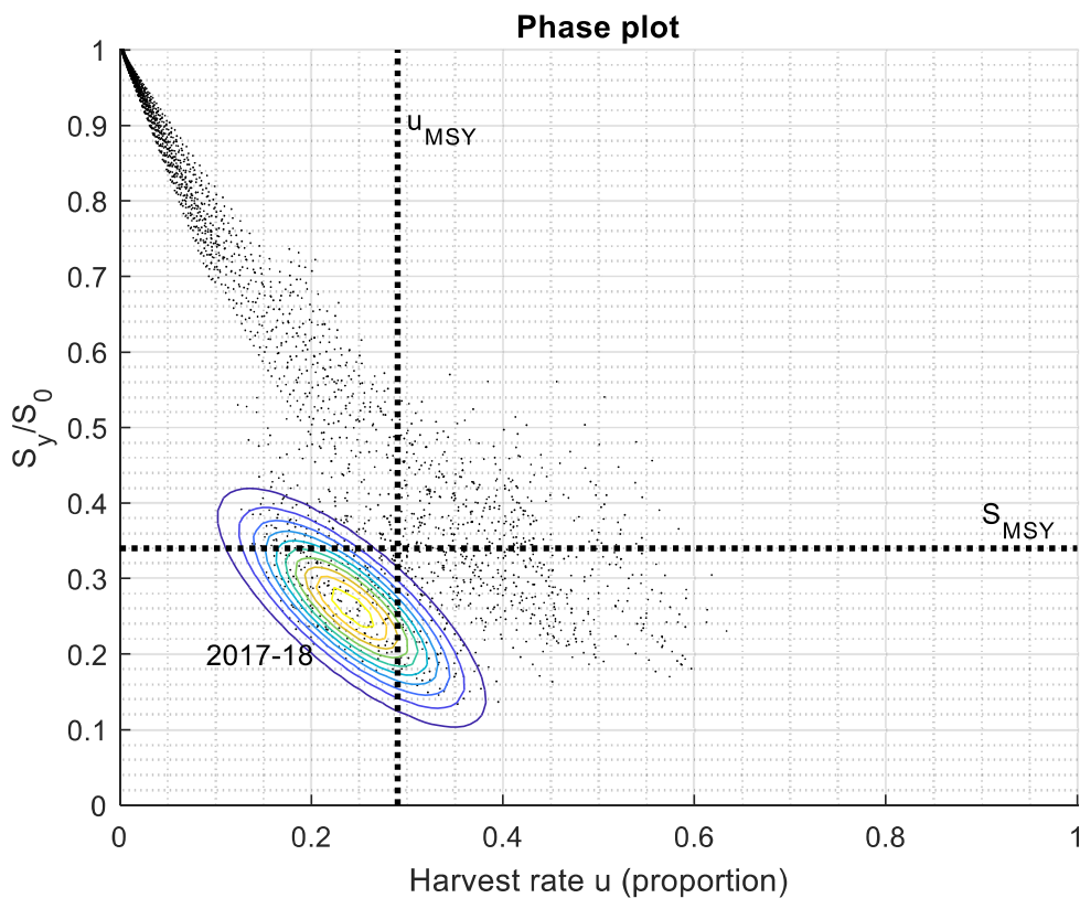
Figure 15. Time series phase plot of fishing harvest rate verse spawning biomass ratio. The contours circle the likely 2017–2018 position. Each dot was a year in each of the 35 analyses.
