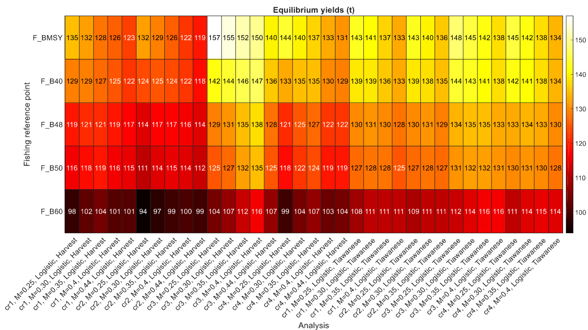
Figure 26. Equilibrium (potential average) yields for each analysis when at their reference point.
