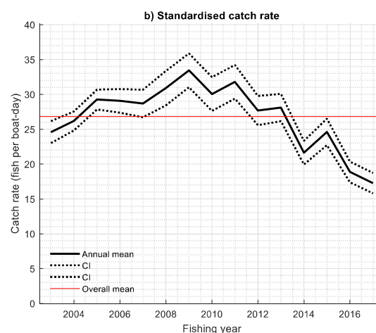
Figure 18. TVH Spanish mackerel average catch rates by fishing year 2003–2017 as predicted from the over-dispersed Poisson GLM. The data included only TSF01 logbook years, including the total hours fished per operation day. The error lines indicate the 95% confidence intervals (CI) on the yearly means.
