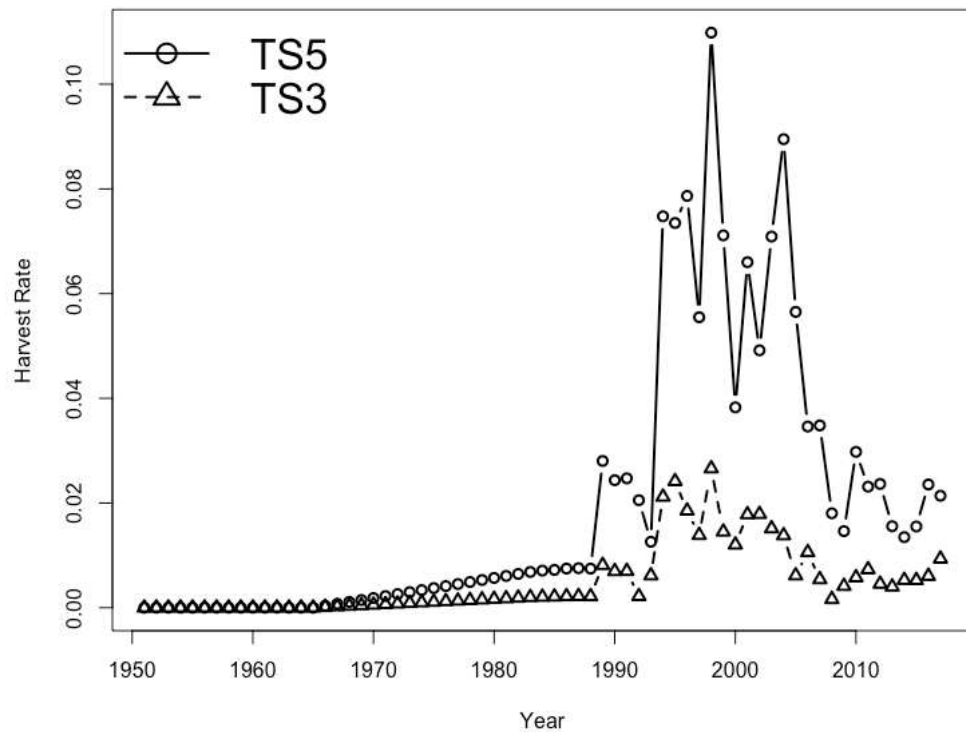
Figure 10: Plot of corresponding estimated fishing mortality in the two regions, with recruitment deviations turned off.
