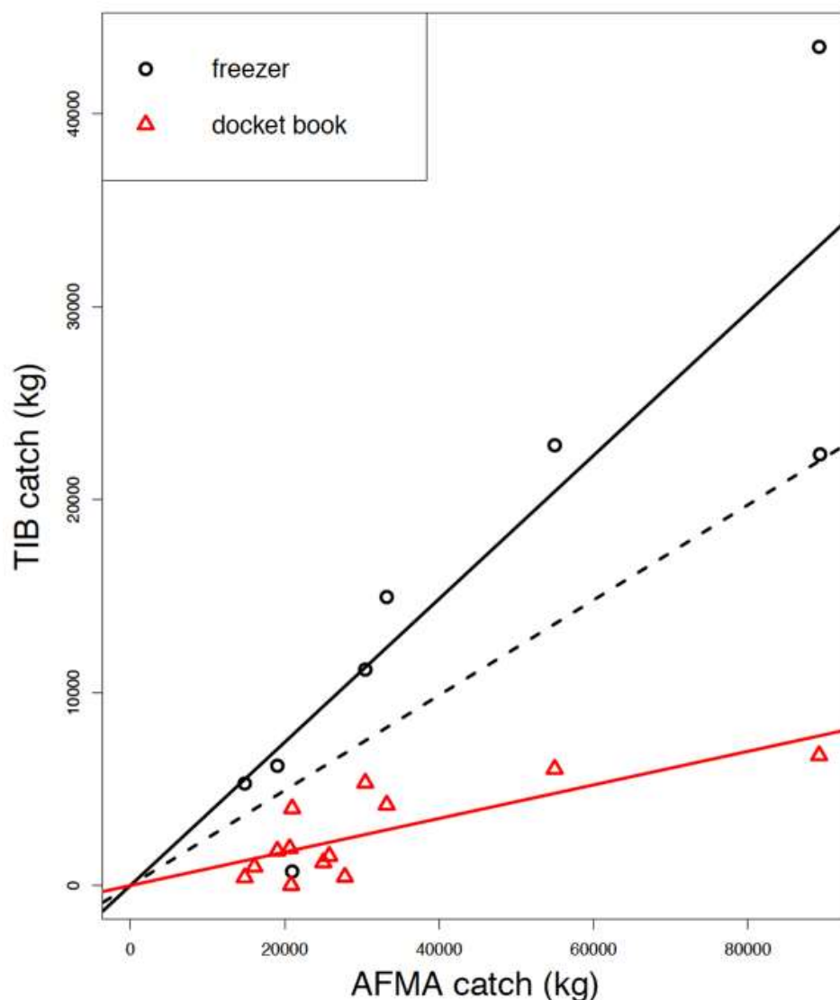
Figure 5: TIB catch from the freezer data set (circles) and docket book data set (triangles) vs sunset fisher catch in the AFMA data set. The lines are the best fitting linear models of TIB catch as a function of AFMA catch. Note that the slope of the line from the model using only the freezer data (black) is 4.2 times higher than the slope from the model using only the docket book data (red).
