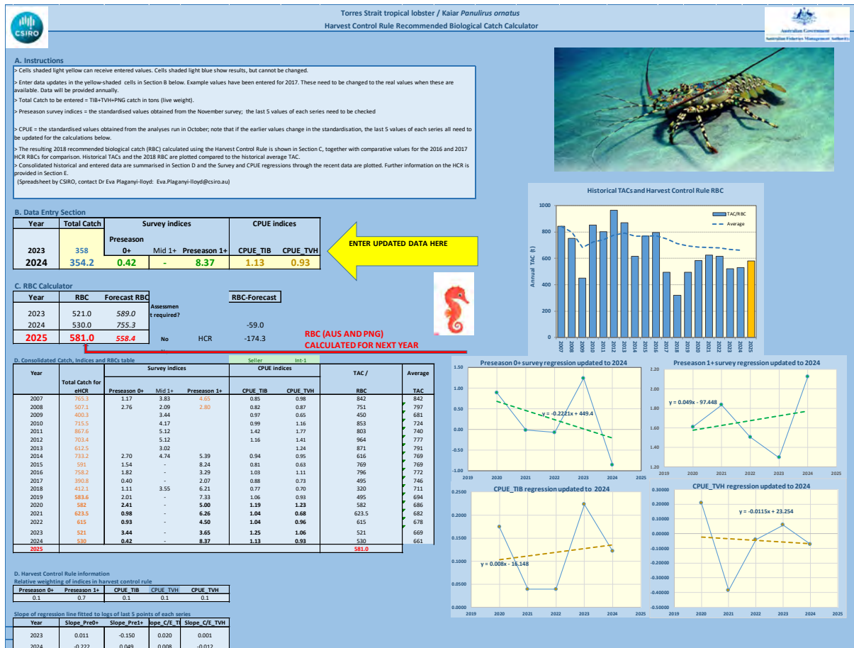
Figure 3-2: Summary of eHCR inputs in December 2024 showing the slopes of fitted regression lines to the log-transformed Preseason 0+ and 1+ indices, as well as the standardised CPUE data for the TIB (Seller model version) and TVH (Int-1 Model version) sectors. Example shown corresponds to the Seahorse eHCR candidate
