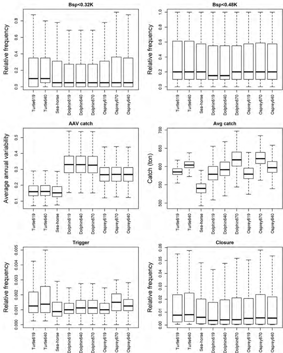
Figure S5- 43: Bar plots of the risk related variables from all simulations for using different rules. The central line shows the median, the box the 75th and 25th percentiles and the whiskers represent the full range of projected values excluding outliers.
